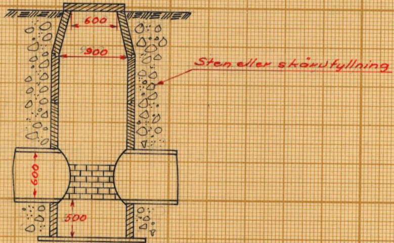
Str 4+68-B
